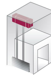
Machine roomless freight elevator 无机房货梯
