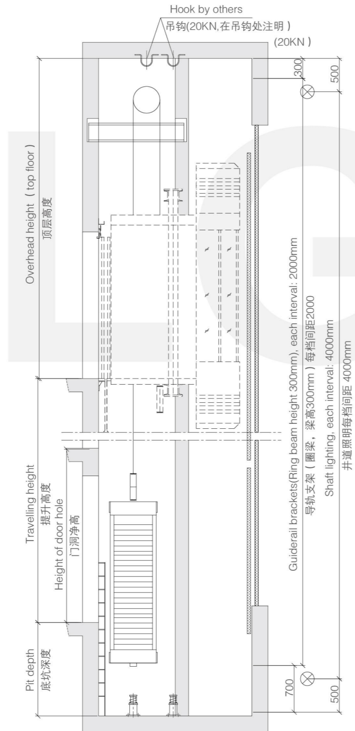
Semicircle type shaft elevational drawing 半圆形井道立面图
